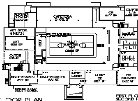
FIRST FLOOR PLAN GRAPHIC SCALE IN FT
